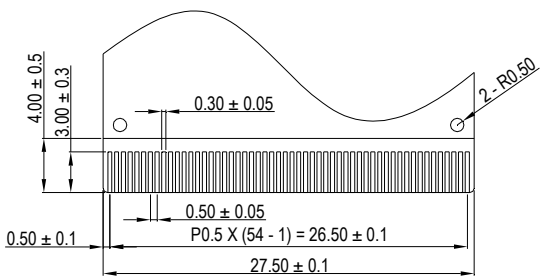
DETAIL B SCALE 2:1
